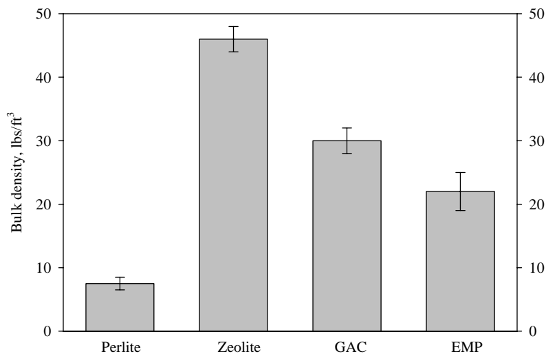
Figure 2. Comparison of media bulk densities.
