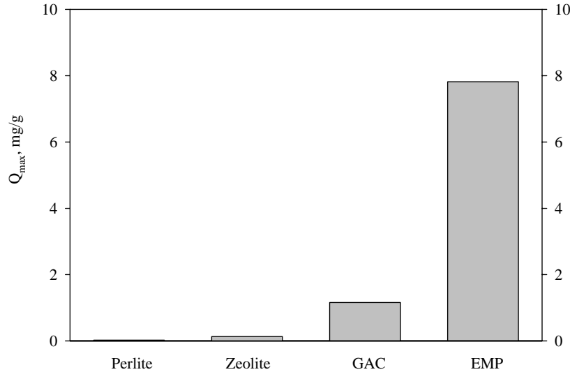
Figure 3. Comparison of media maximum phosphate adsorption capacities by isotherms.
