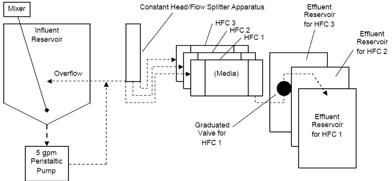
Figure 1. Illustration of the testing apparatus for breakthrough experiment. Dashed lines represent flow. Graduated valves and effluent flow vectors for horizontal flow columns (HFC) of 2&3 have been left out for clarity.
