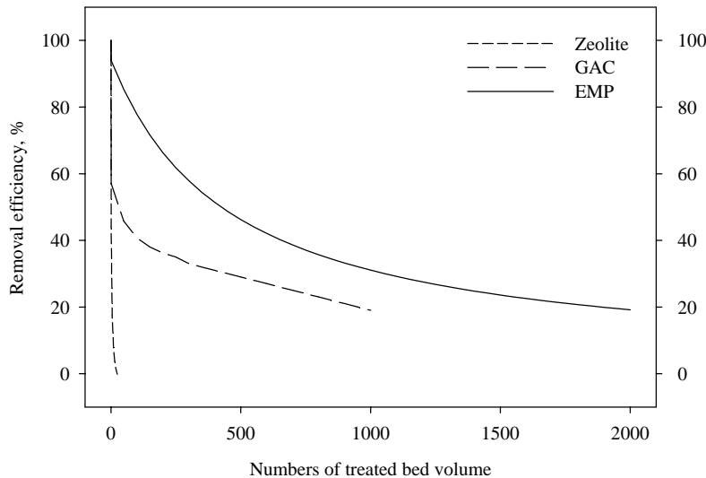
Figure 4. Phosphate adsorption breakthroughs for GAC, Zeolite and EMP media
