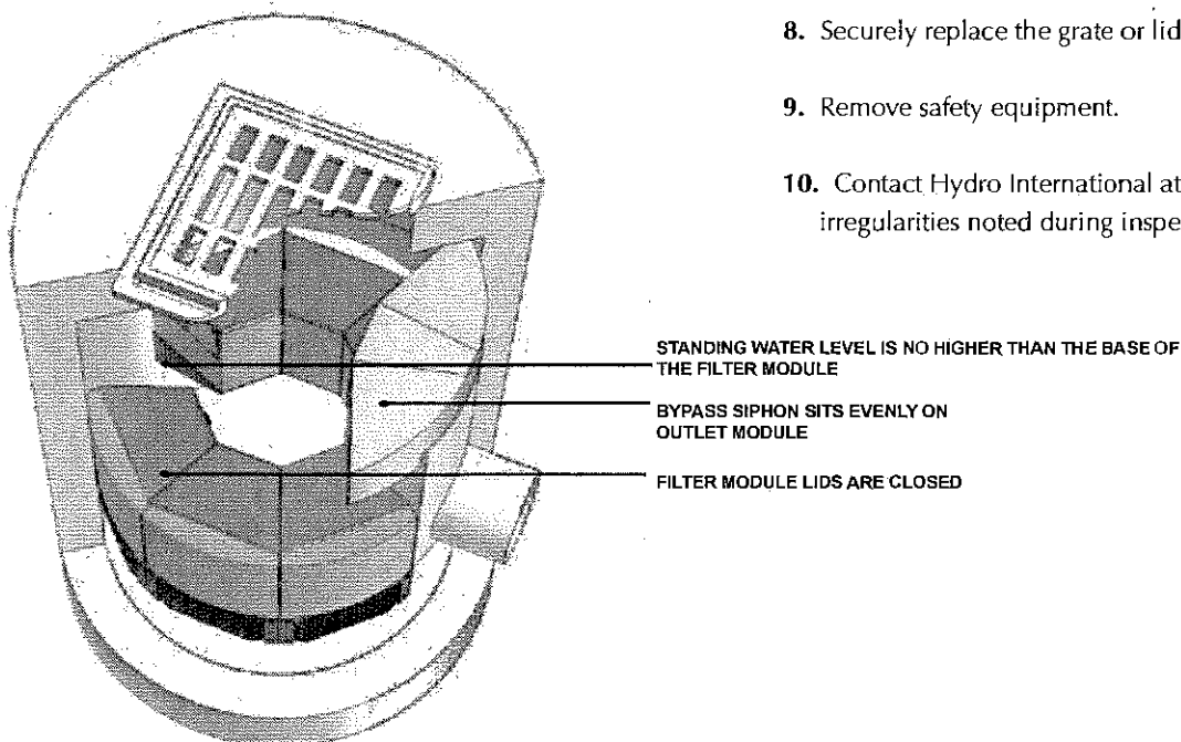
Figure 3: Inspection view of the Up-Flo Filter
