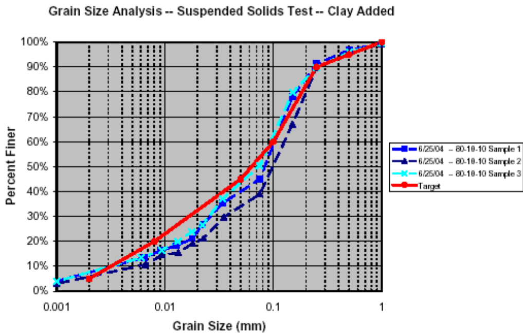
Figure 3. Comparison of the size distributions of three mixes (batches) with the target size distribution. The dashed lines are samples from three different mixes (batches) with similar proportions of sediments. The 5% clay was hypothetically added to the size distributions of the samples.
