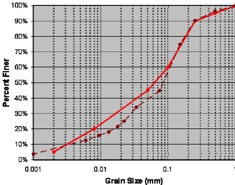
Figure 4. Comparison of the size distributions of the average of three mixes (batches) with the target size distribution.
