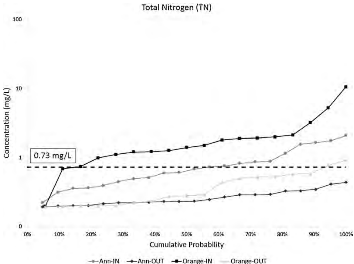
Fig. 6. Cumulative probability plots for effluent TN concentration with “good” water quality threshold in NC coastal plain as described by McNett et al. (2010).
