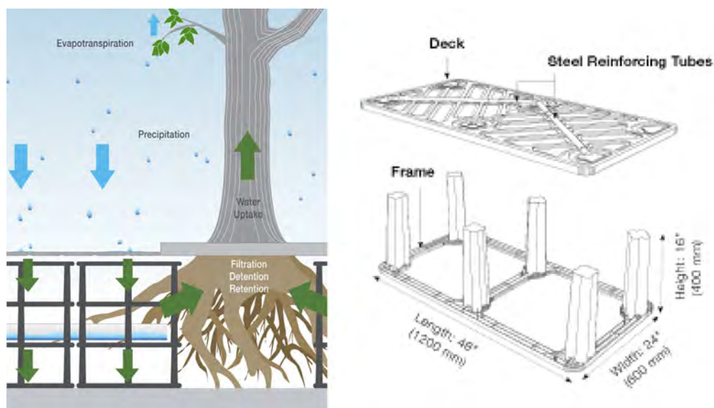
Fig. 1. Schematic and detail of the Silva Cell™ suspended pavement system (image courtesy of DeepRoot Green Infrastructure, LLC).
