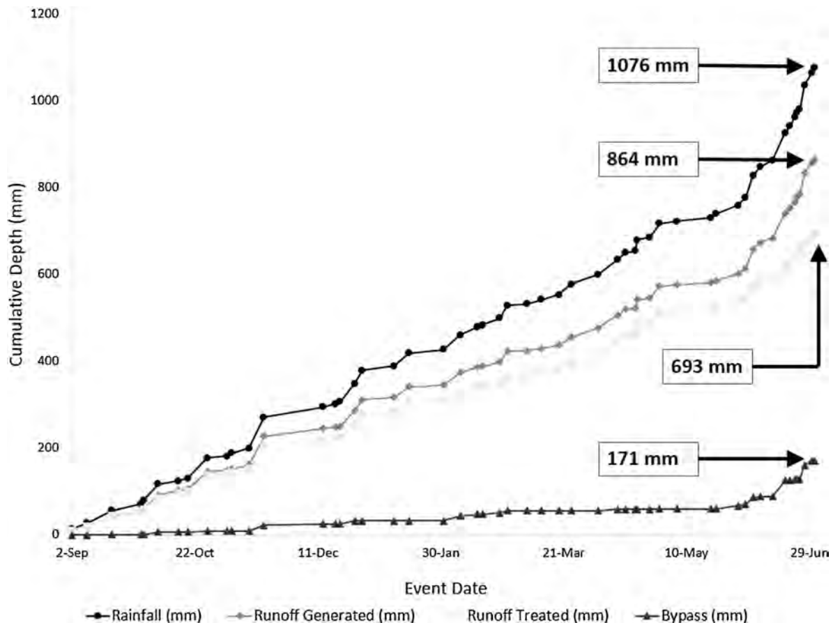
Fig. 3. Cumulative fate of runoff at the Ann Street site.
