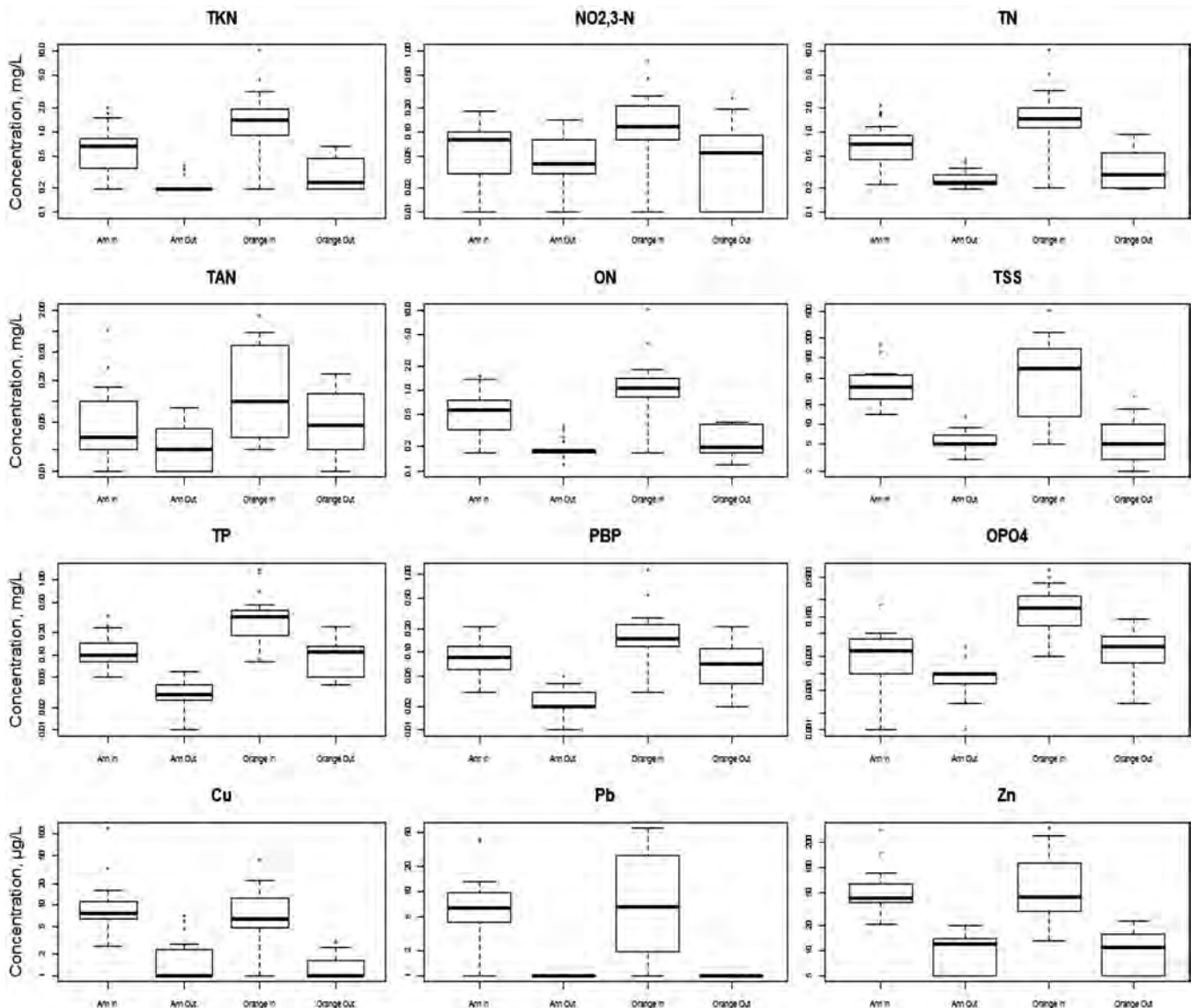
Fig. 5. Boxplot summary of pollutant concentration distributions for Ann Street and Orange Street sites in Wilmington, NC.
