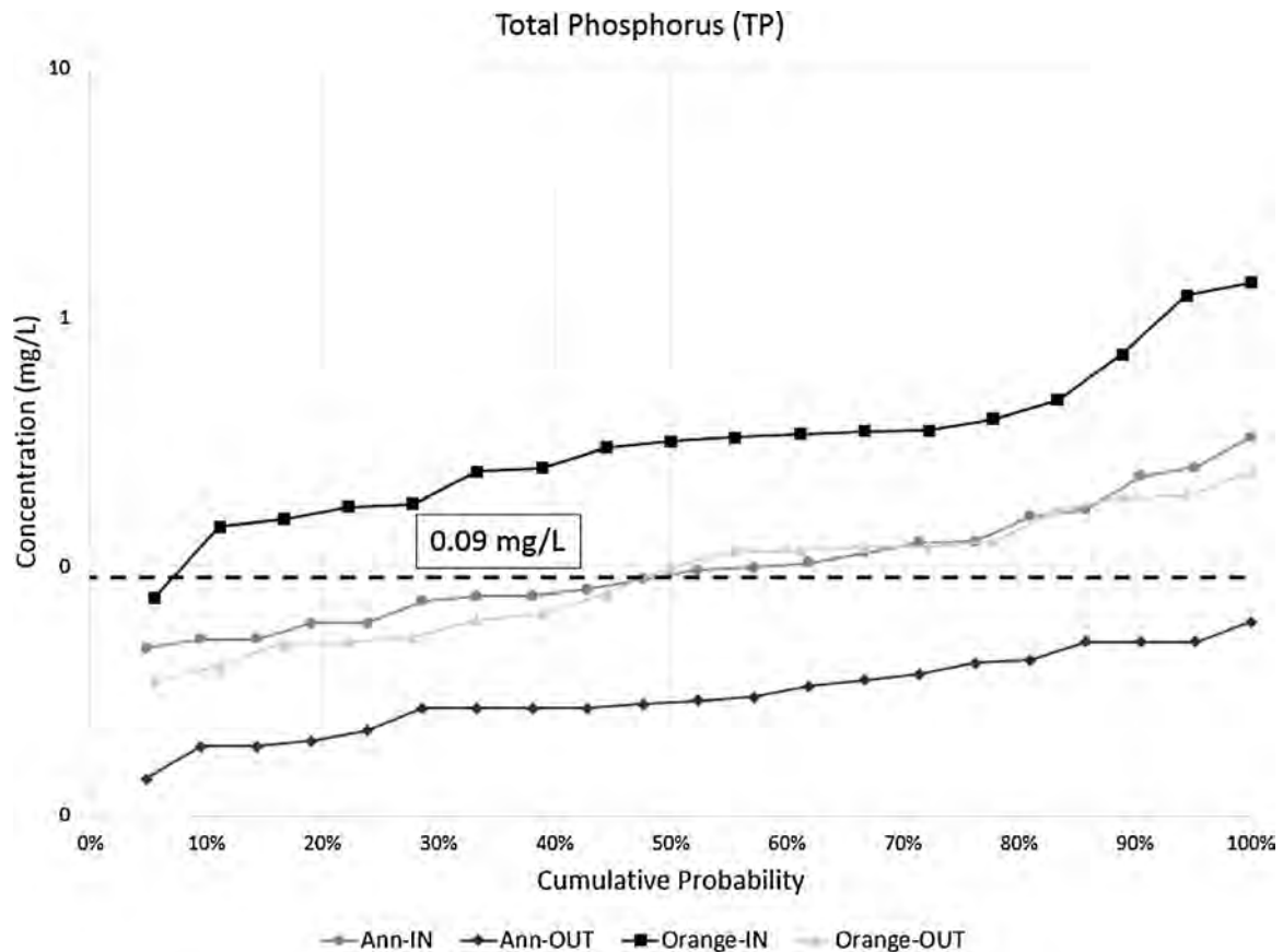
Fig. 7. Cumulative probability plots for effluent TP concentration with “good” water quality threshold in NC coastal plain as described by McNett et al. (2010).
